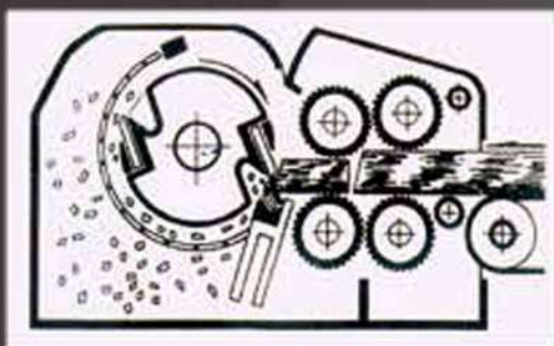
PX Disc Wood Chipper
